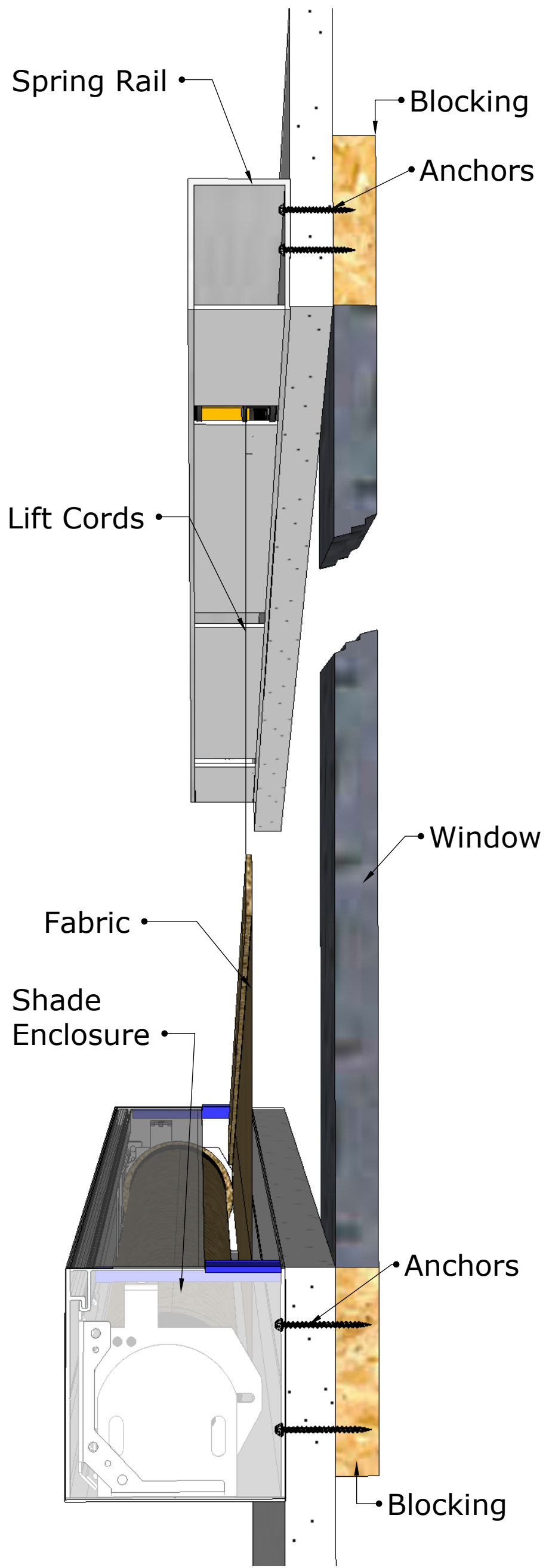
Outside Mount Typical
